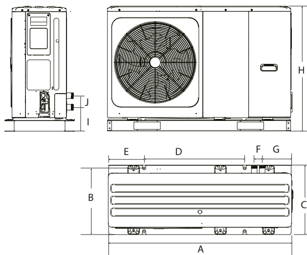
8/10/12/14/16 kW (dimenzije v mm)
