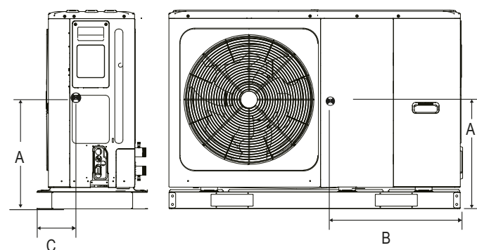
8/10/12/14/16 kW (dimenzije v mm)
